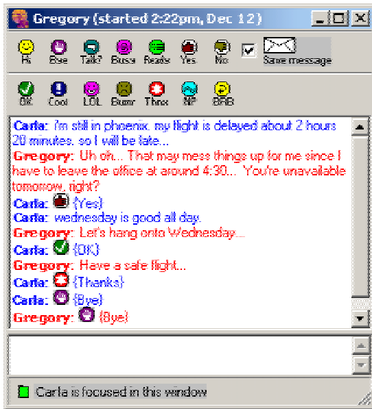
Figure 3. Text Message window on PC Hubbub.
